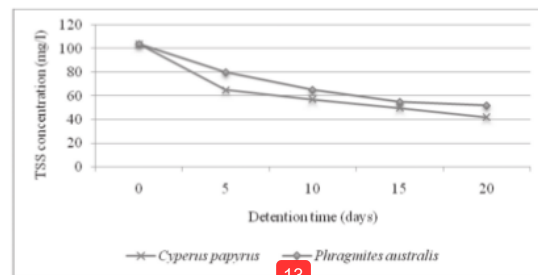
Fig. 3. TSS elimination in constructed wetland using various plant species
