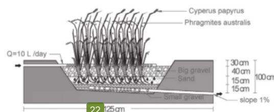
Fig. 1. Sub surface flow constructed wetland
